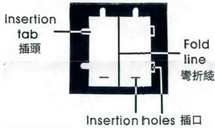
Schematic drawing of sheet metals (two pieces of sheet metals). 金屬片示意圖 (有2片金屬)
